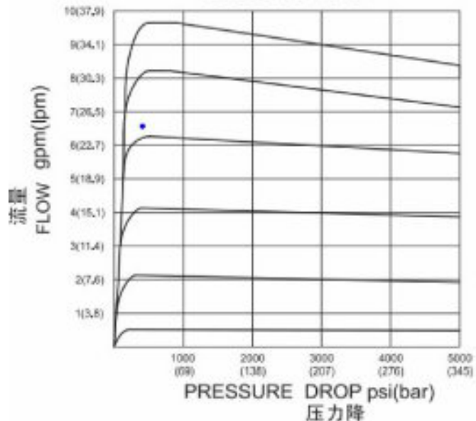
① to ② 压力流量曲线 Regulated Flow vs. Pressure Drop 46cSt oil @ 40°C
